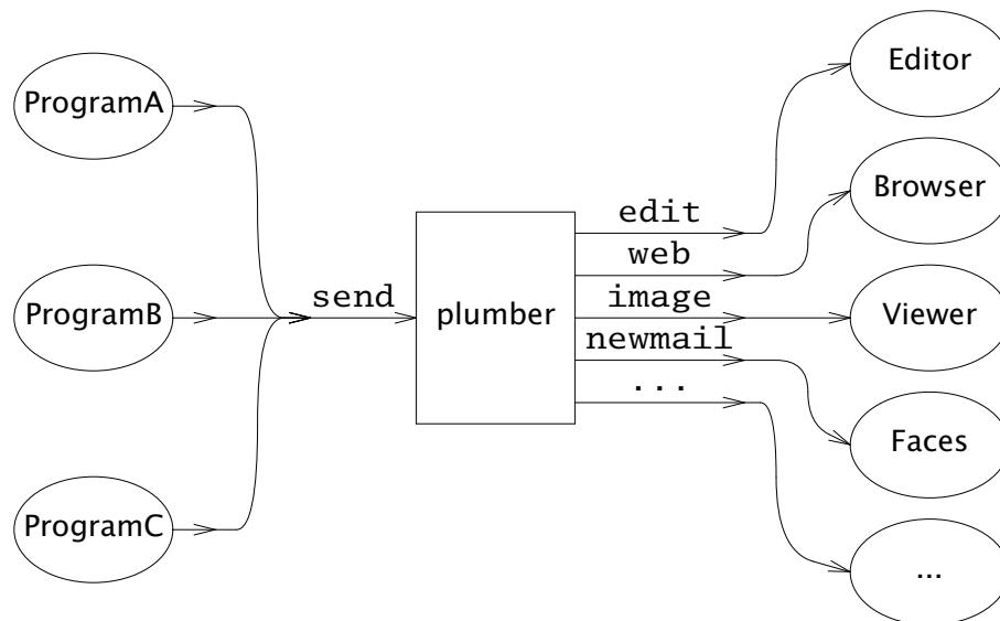
Figure 1. The plumber controls the flow of messages between applications. Programs write to the file send and receive on 'ports' of various names representing services such as edit or web . Although the figure doesn't illustrate it, some programs may both send and receive messages, and some ports are read by multiple applications.
